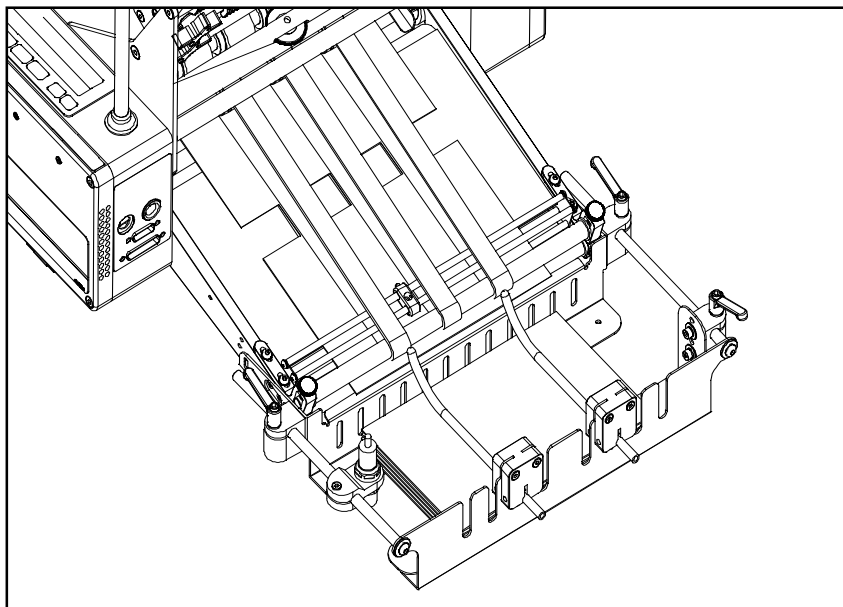
Fig. 1. SMCT 350 M Catch Tray on MFT 350 ED Friction Feeder
