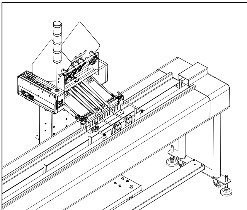
Fig. 2. The SMCT style Catch Tray in use with the HSC-3 High Speed Collator
